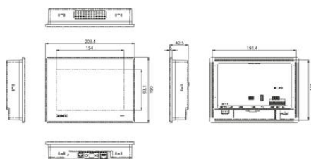
Panel Cut Out Dimensions: 192 x 138.5 mm (7.56" x 5.45")
