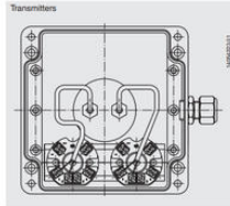
Terminal on transmitter on terminal
