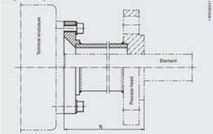
Straight tube design
