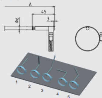
Tightening strap
