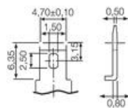
Faston flat connector 4,8 mm
