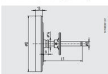
Smooth connection, with sliding plastic flange
