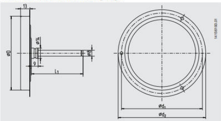
Smooth connection, with rear mounting flange
