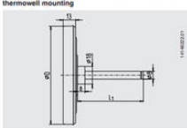
Smooth connection, with 18 mm collar diameter for thermowell mounting
