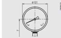
Model R74.100, lower mount, standard version
