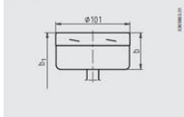
Model A74.100, back mount, standard version
