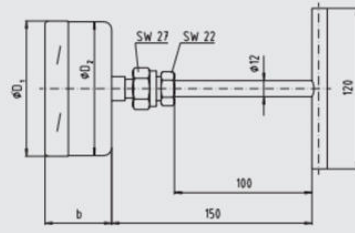
Model A73, with contact bulb Back mount (BM)
