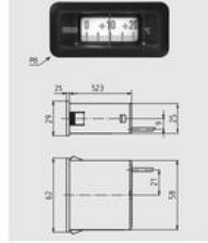
Model TF01-059KF (radius 5 mm)
