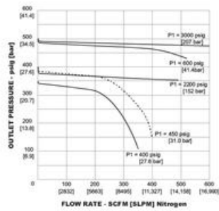
CP3220 - Lower P1 pressures (CP321402280-001)
