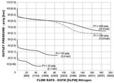
CP3220 - Lower P1 pressures (CP321402280-001)
