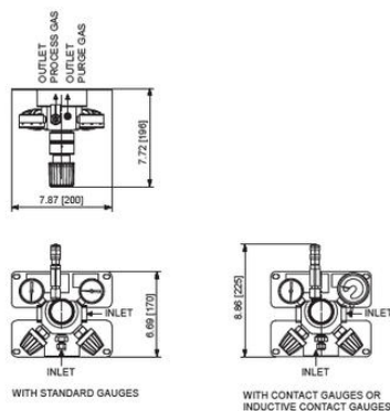
HIGH PRESSURE PANEL FOR 1 CYLINDER
