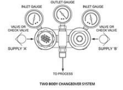
TWO BODY CHANGEOVER SYSTEM
