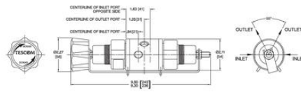
CR441800 SERIES CHANGEOVER SYSTEMS (HIGH PRESSURE)
