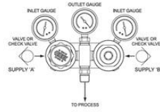
TWO BODY CHANGEOVER SYSTEM
