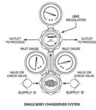
SINGLE BODY CHANGEOVER SYSTEM
