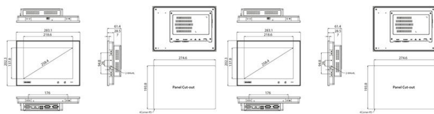
TPC-1051WP Panel Cut-out Dimensions: 274.6 x 193.8 mm
