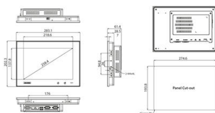
TPC-1051WP Panel Cut-out Dimensions: 274.6 x 193.8 mm
