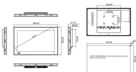
Panel Cut-out Dimensions: 479.30 x 300.30 mm (18.87" x 11.82")
